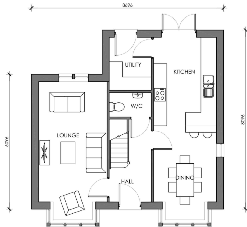
GROUND FLOOR
