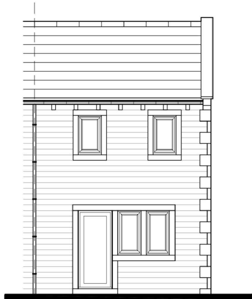
REAR ELEVATION
