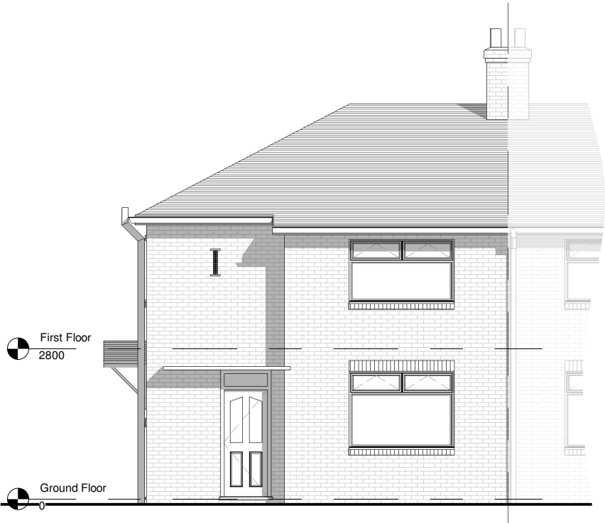
North Elevation - Existing 1 : 100
