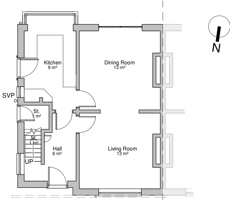
Ground Floor Plan - Existing 1 : 100
