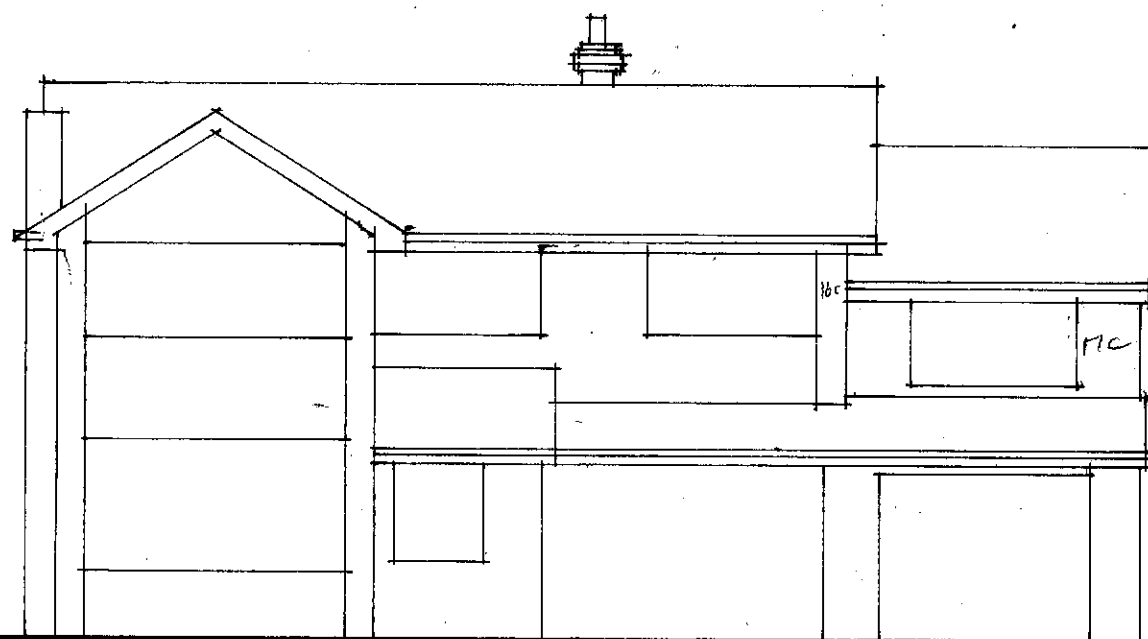
FRONT 1:100
