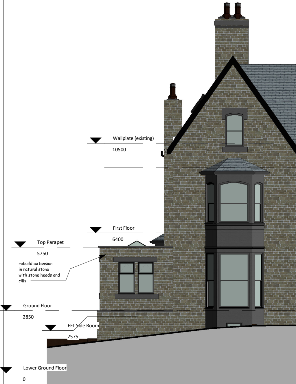
11 Front Proposed 1 : 100
