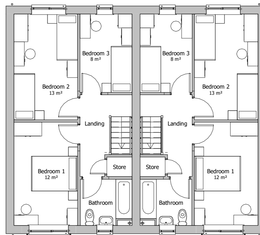
Plots 7 and 8 First Floor Plan 1 : 100
