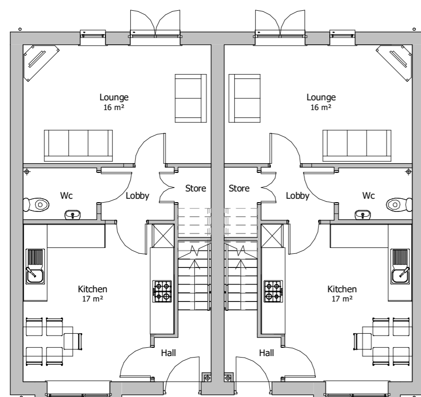
Plots 7 and 8 Ground Floor Plan 1 : 100
