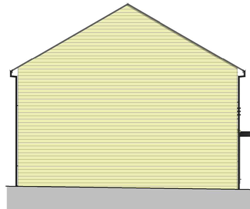
Plot 7 Side Elevation 1 : 100
