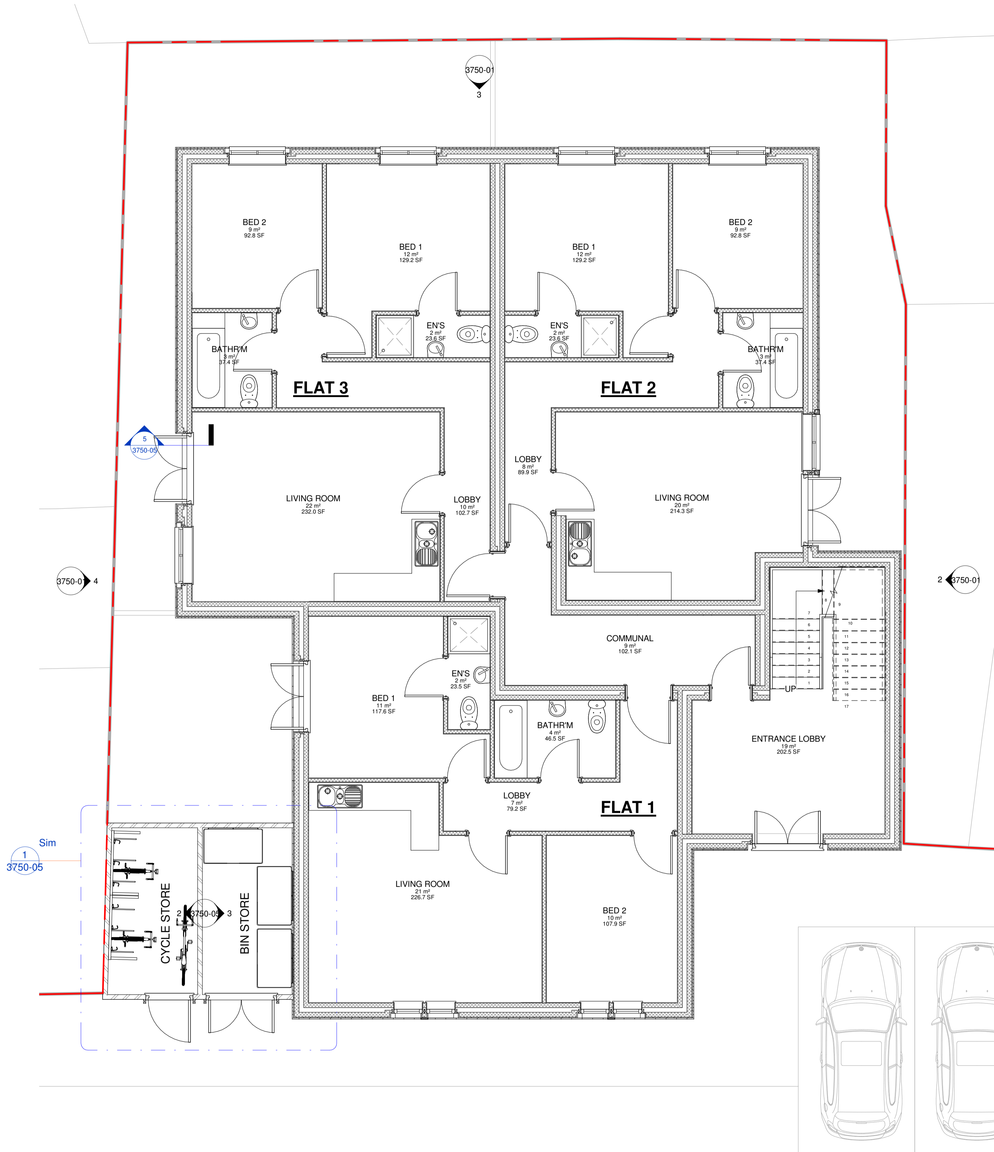
1 GF FFL - PROPOSED 1 : 50
