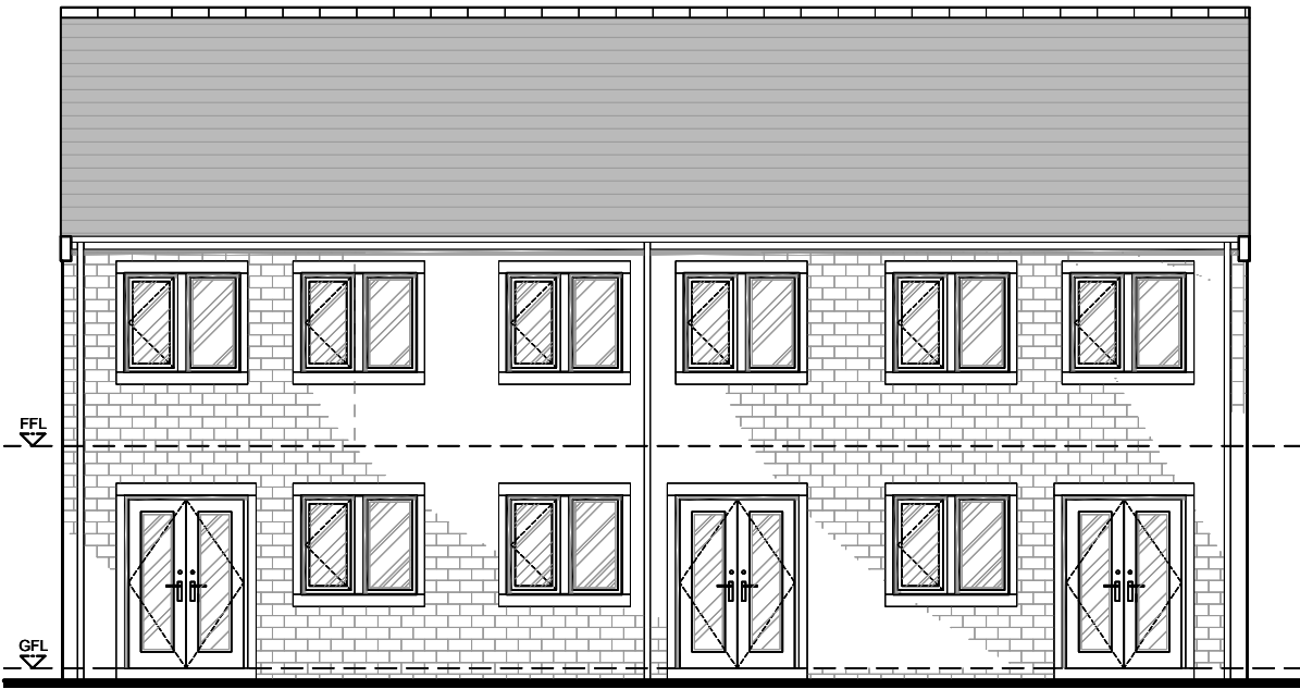
REAR ELEVATION
