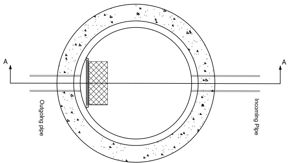
TYPICAL 1200mm FLOW CONTROL CATCHPIT MANHOLE
