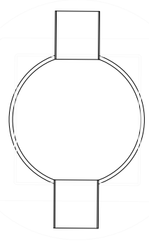
TYPICAL 600mmØ CATCHPIT INSPECTION CHAMBER (MAXIMUM DEPTH 1200MM) SCALE 1:20
