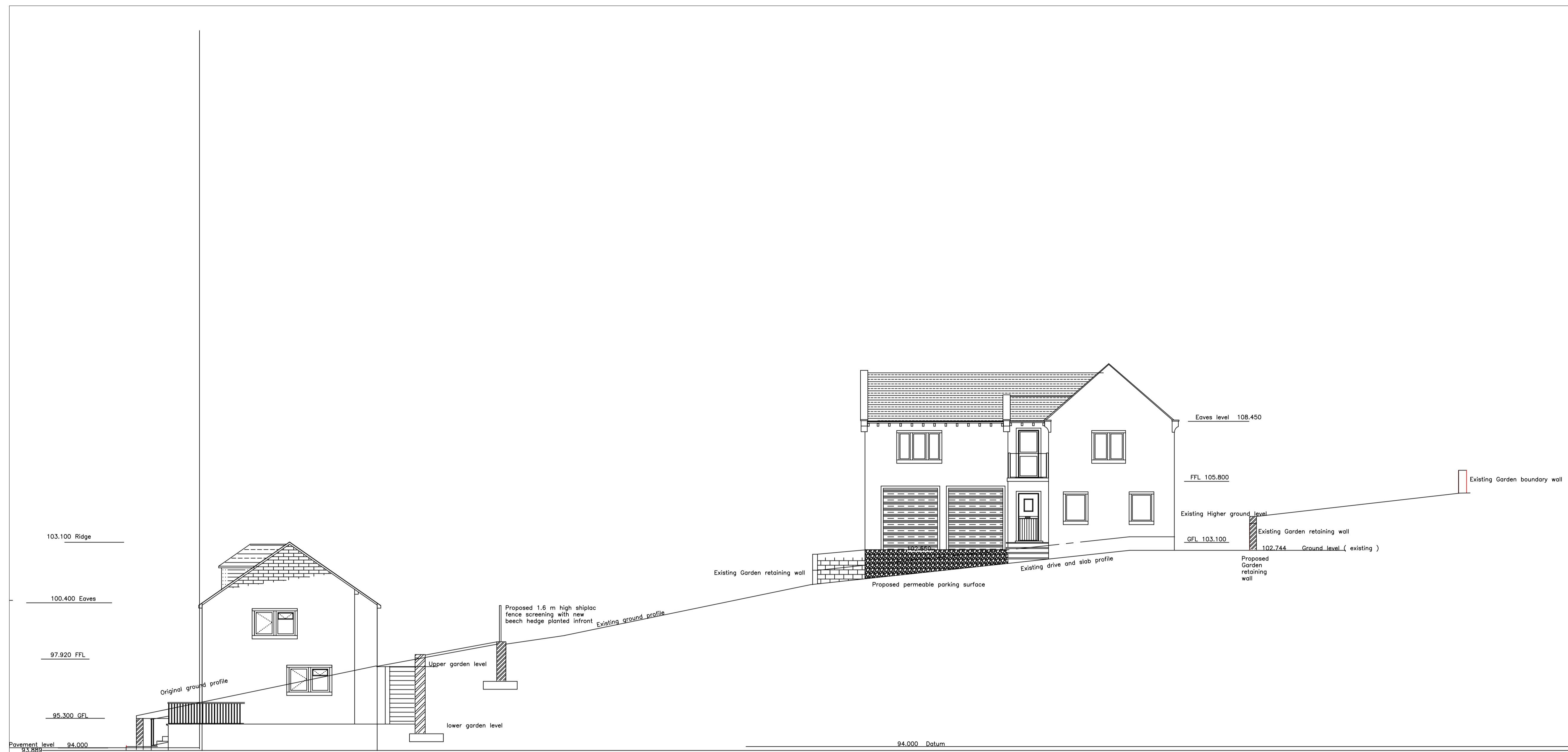
Proposed Stepped Section Showing Existing Ground Levels & Proposed levels High for Beeches Developments
