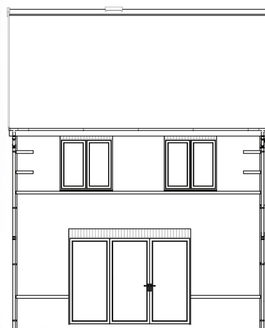
REAR ELEVATION
