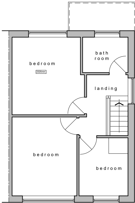
FIRST FLOOR PLAN - EXISTING 1:100
