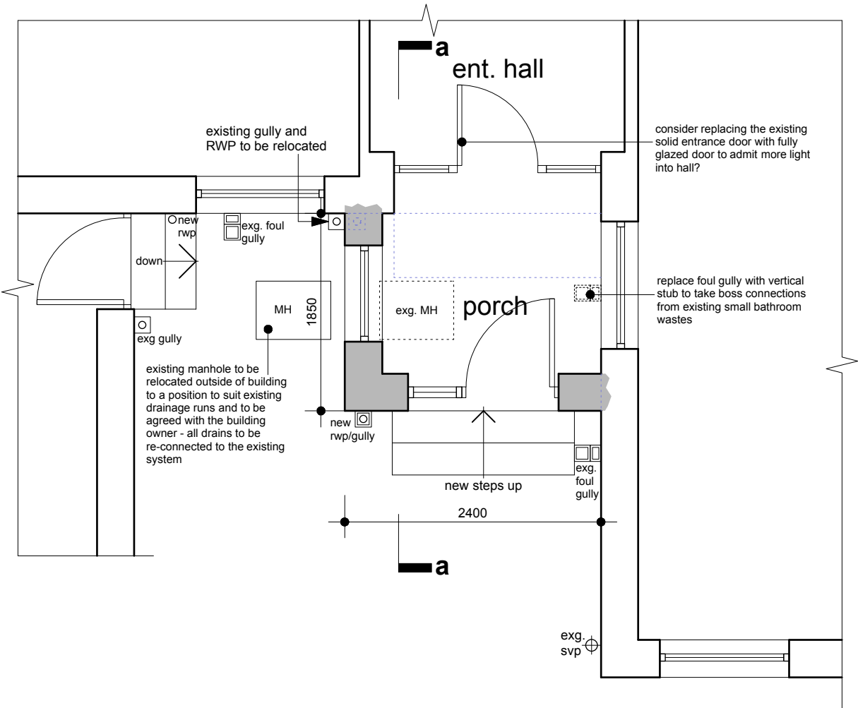
partial ground floor plan
