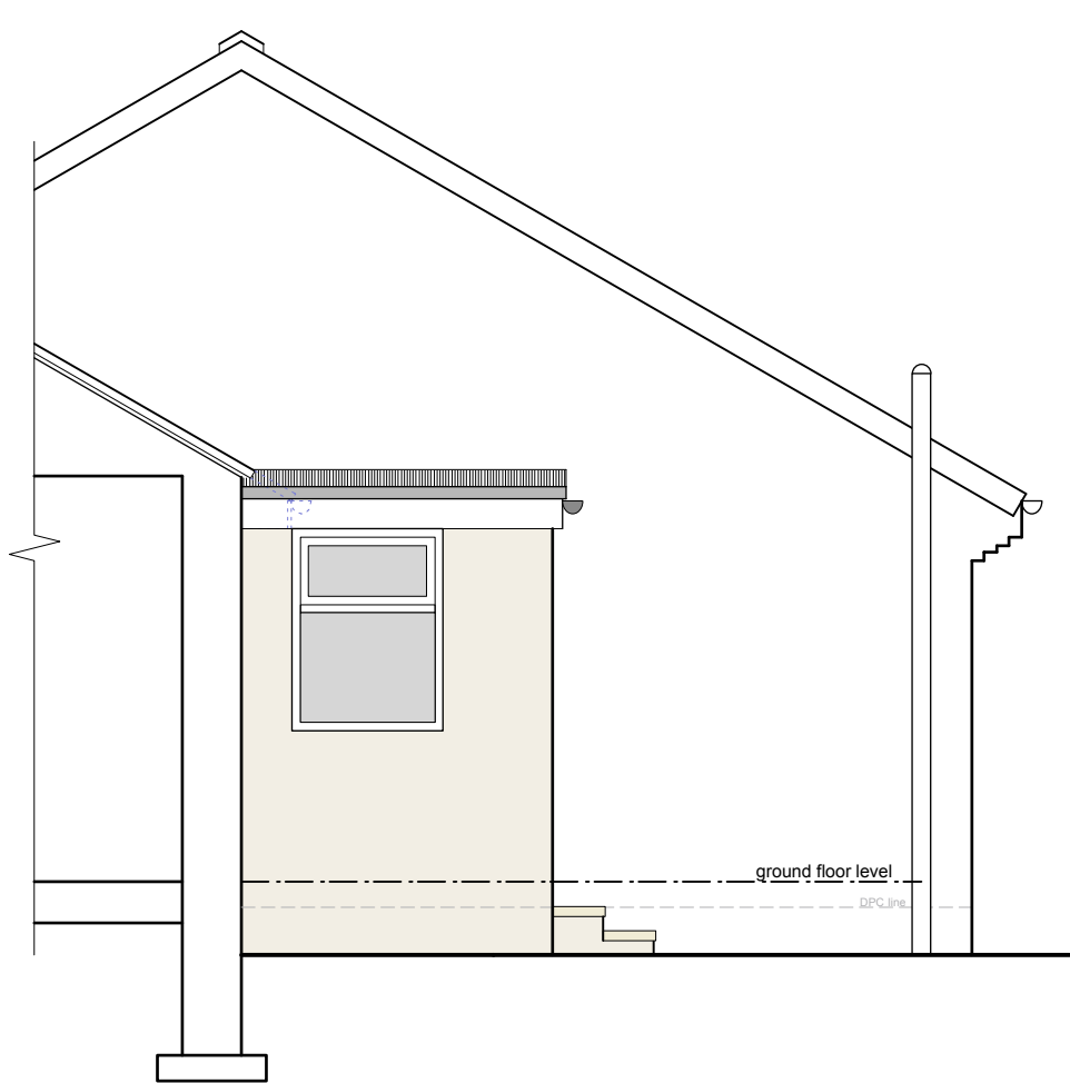
side elevation
