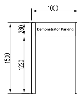
R 5 x Nova Direction Sign #2 TEXT FREESTANDING NON-ILLUMINATED HEIGHT: 1500 WIDTH: 1000 DOUBLE SIDED FIX TO: NEW FOUNDATION SIDE ONE: Demonstrator Parking SIDE TWO: Demonstrator Parking
