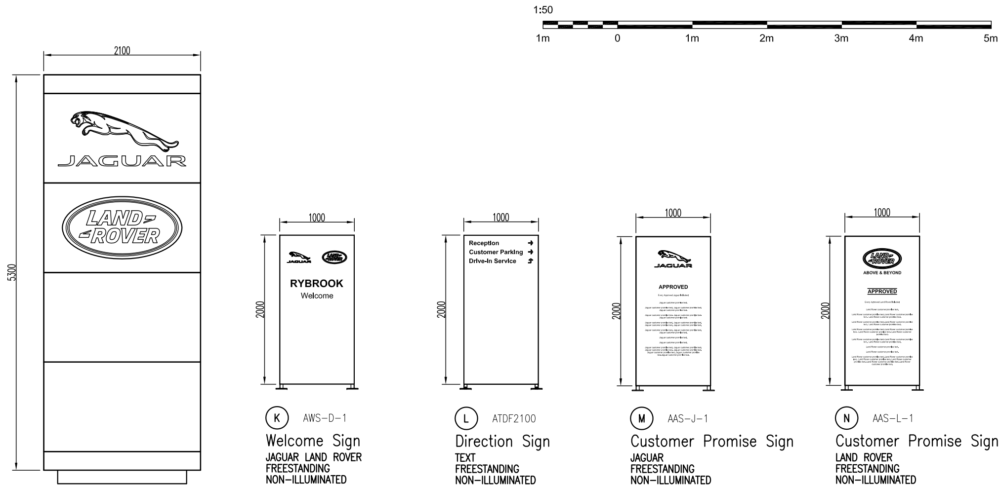
A APL-D5 Dual Brand Pylon JAGUAR LAND ROVER ILLUMINATION: LOGOTYPES HEIGHT: 5300 WIDTH: 2100 BASE: NEW CONCRETE FOUNDATION AND BASE CAGE REQUIRED NOTE: 10 AMP
