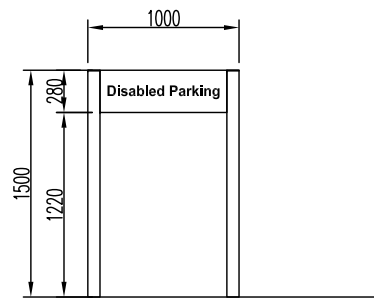
Q 2 x Nova Direction Sign #1 TEXT FREESTANDING NON-ILLUMINATED HEIGHT: 1500 WIDTH: 1000 SINGLE SIDED FIX TO: NEW FOUNDATION Disabled Parking NOTE: SIGNAGE NOT REQUIRED IF APPROPRIATE GROUND MARKINGS ARE PROVIDED
