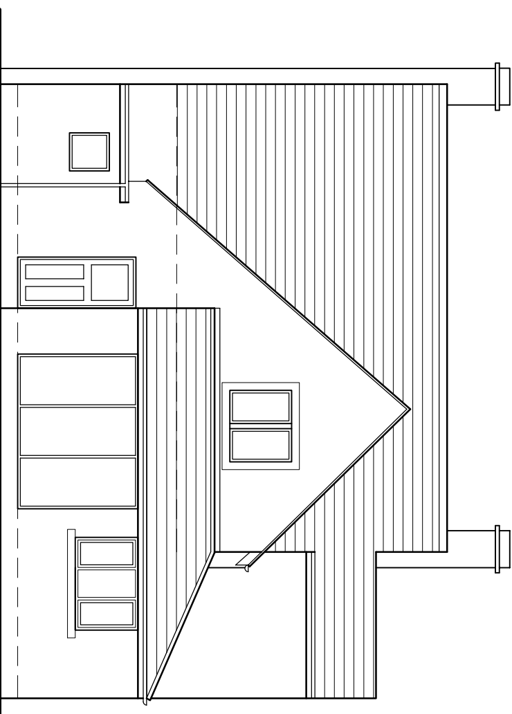
Rear Elevation
