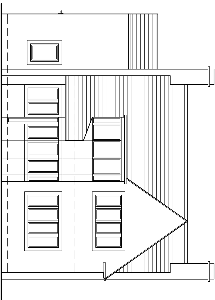
Front Elevation
