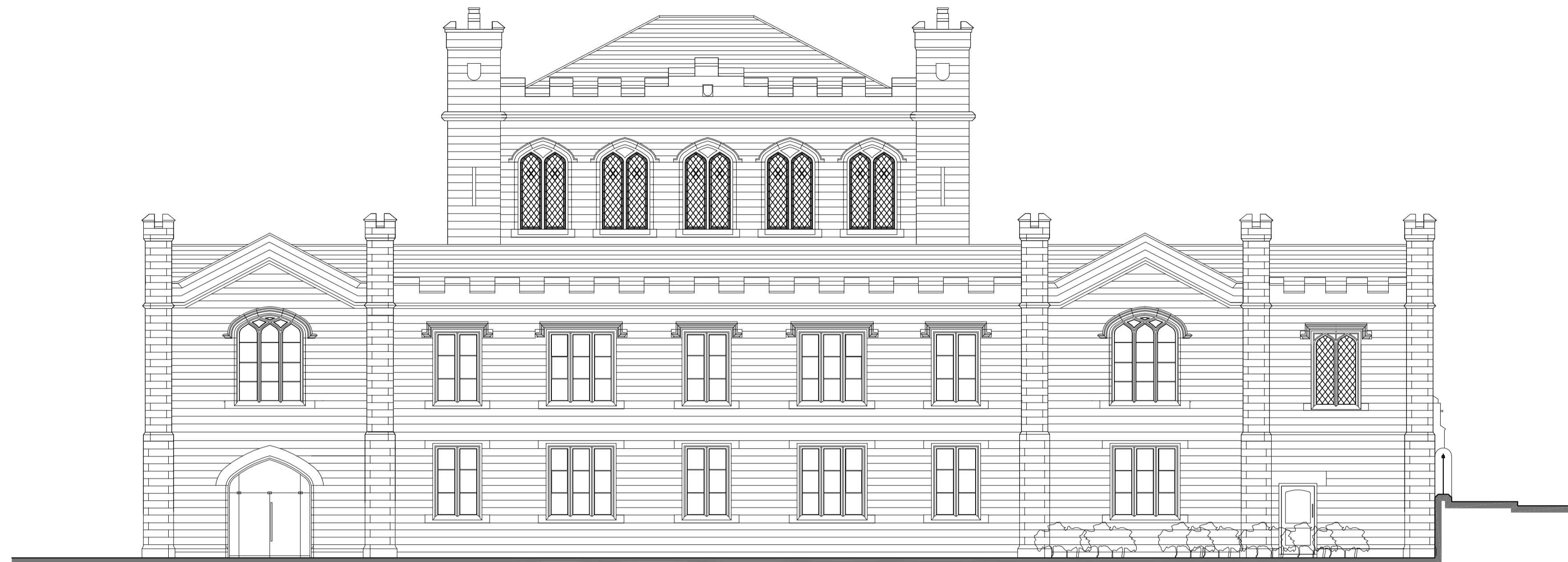
ELEVATION FACING NORTH WEST (no changes are proposed)
