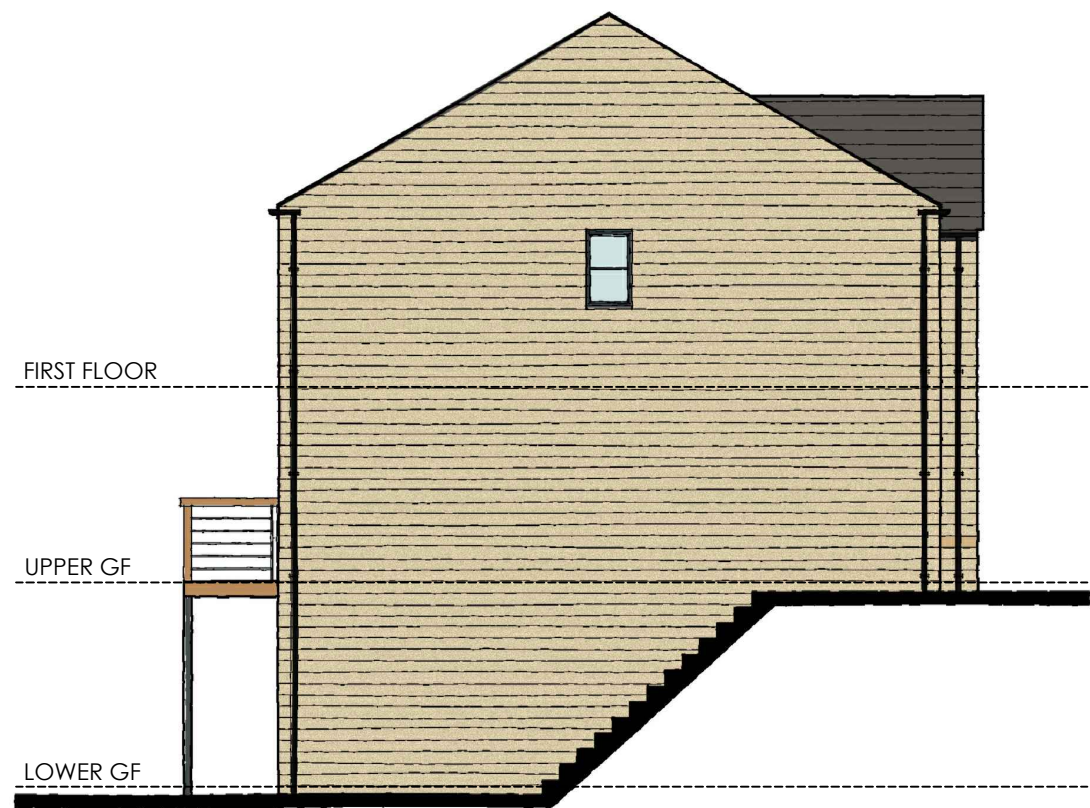
PLOT 16 SIDE ELEVATION
