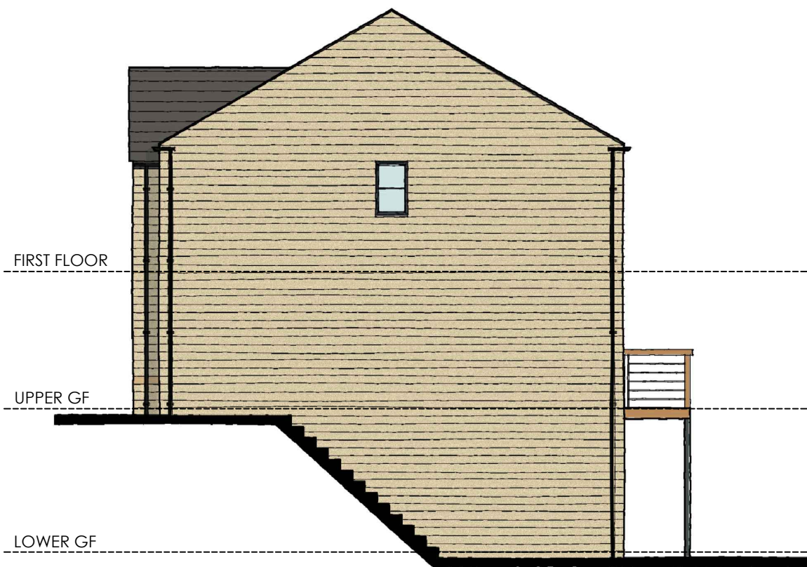
PLOT 17 SIDE ELEVATION
