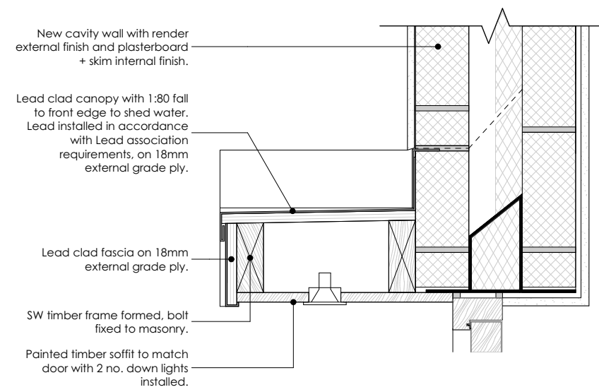
Canopy Detail 1:5
