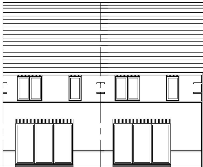
REAR ELEVATION Lorton (mid)
