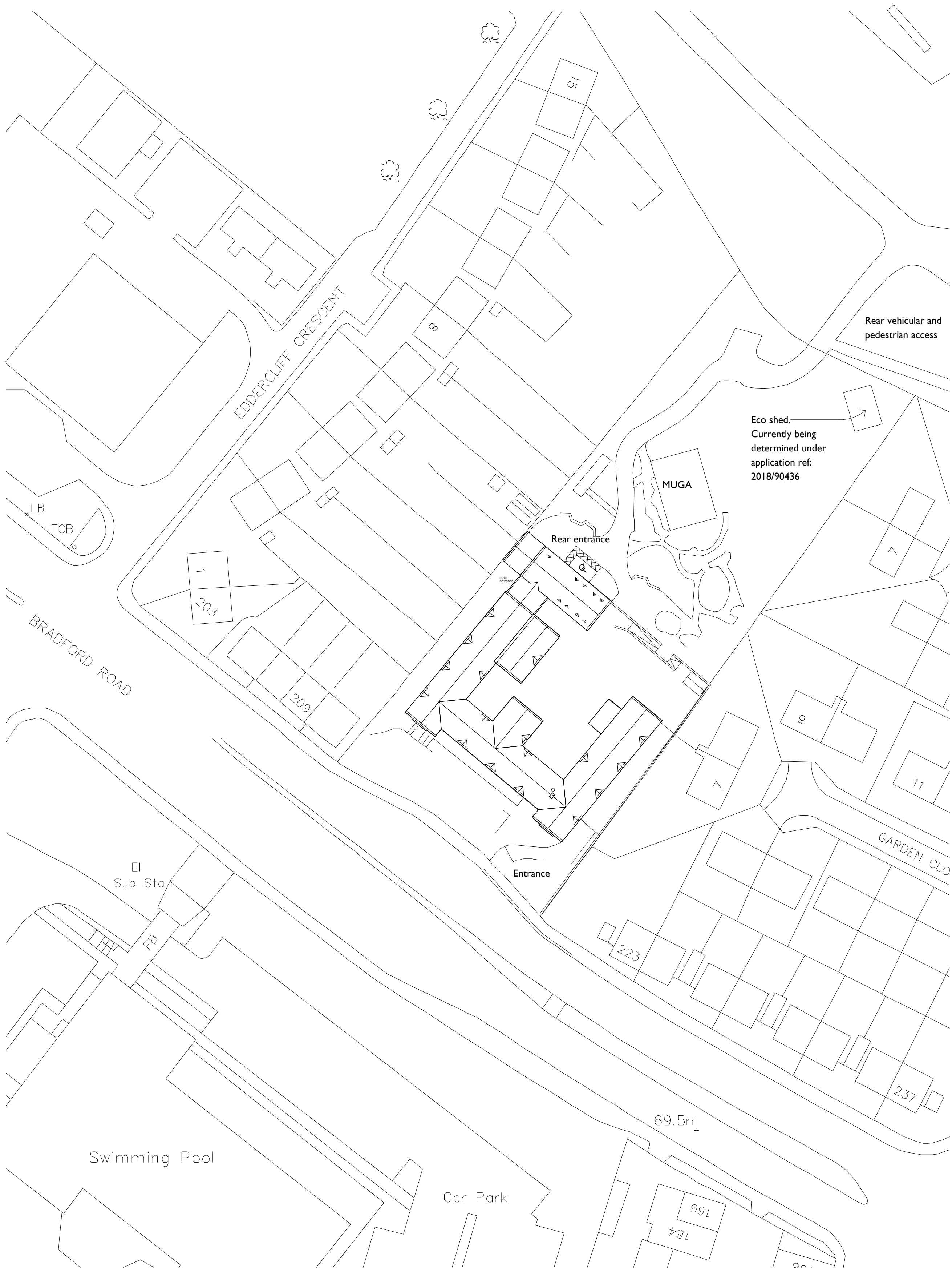
Existing Site Layout 1:300
