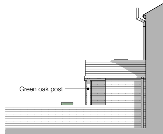
Porch north elevation 1:100
