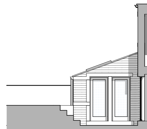
Sun room south elevation 1:100
