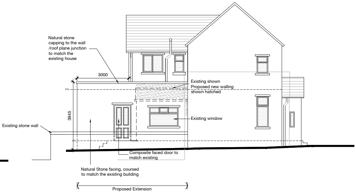
NORTH-WEST ELEVATION
