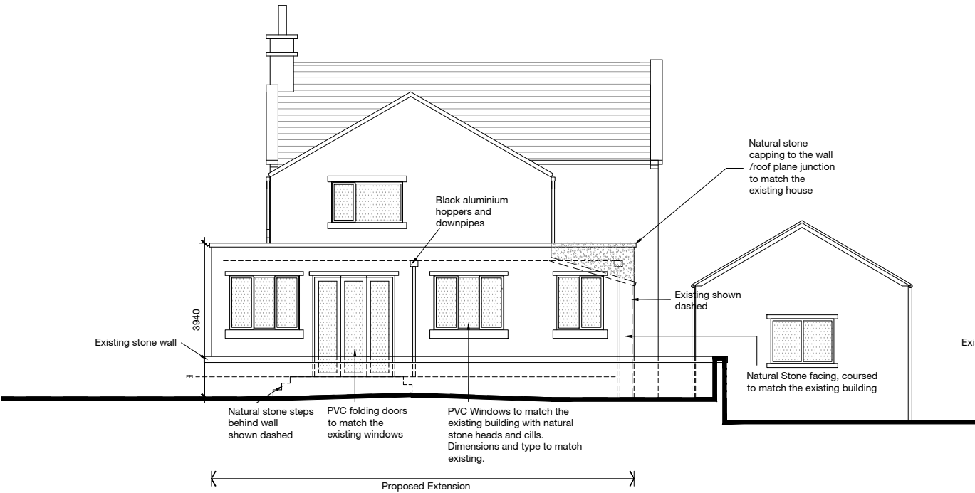
NORTH-EAST ELEVATION
