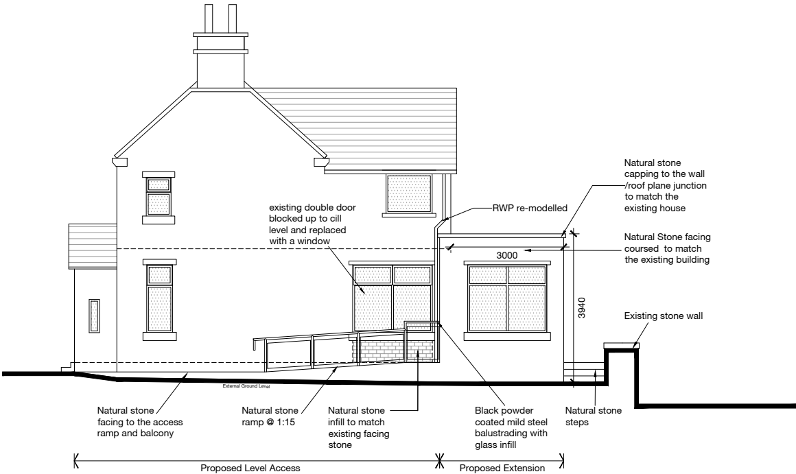
SOUTH-EAST ELEVATION
