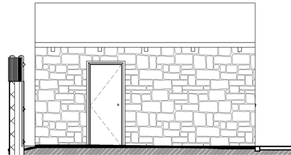
north side elevation 1 : 50
