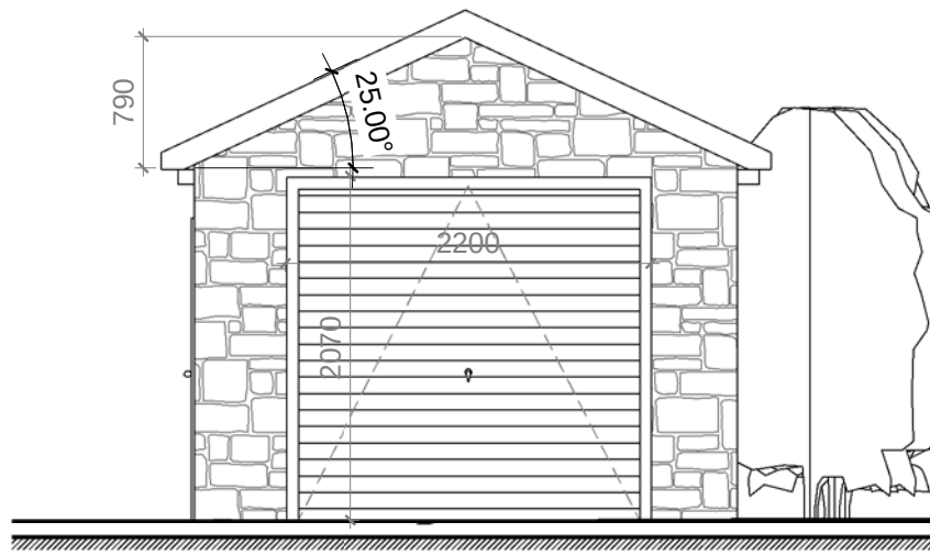
west front elevation 1 : 50
