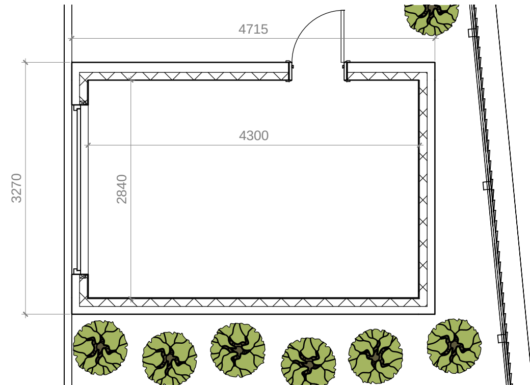
proposed plan view 1 : 50
