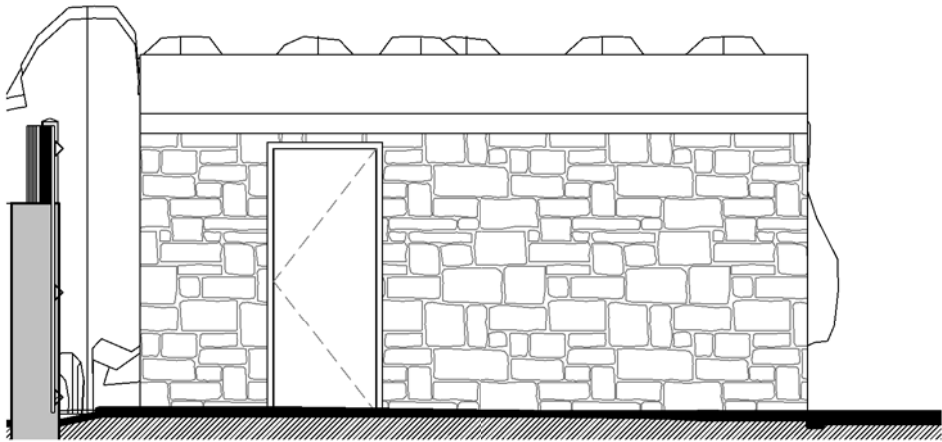
north side elevation 1 : 50
