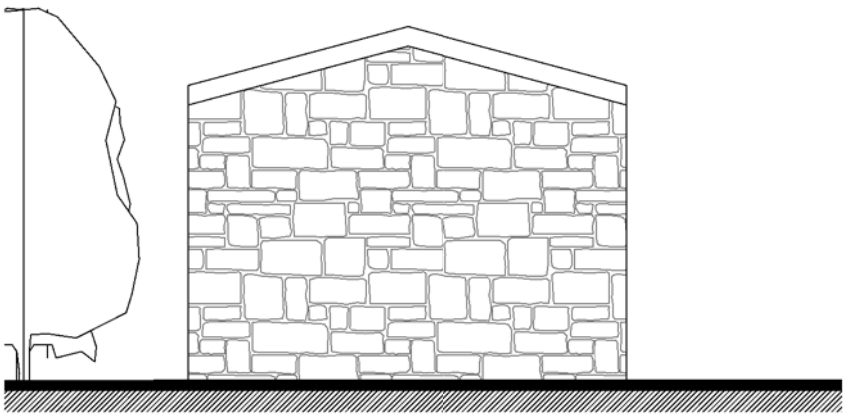
east side elevation 1 : 50
