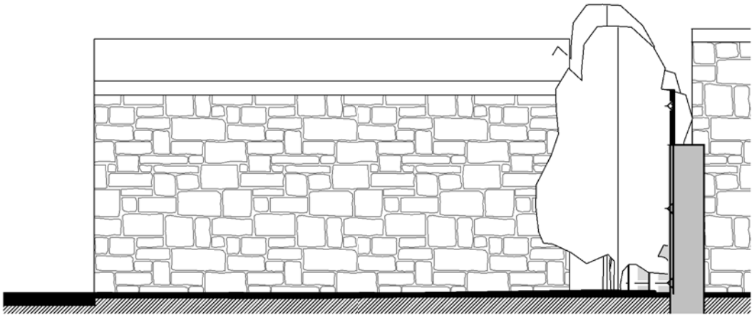
south side elevation 1 : 50
