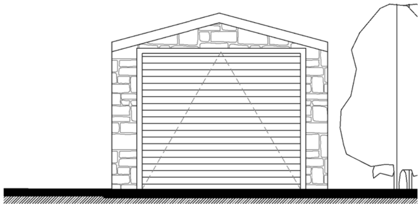
west front elevation 1 : 50
