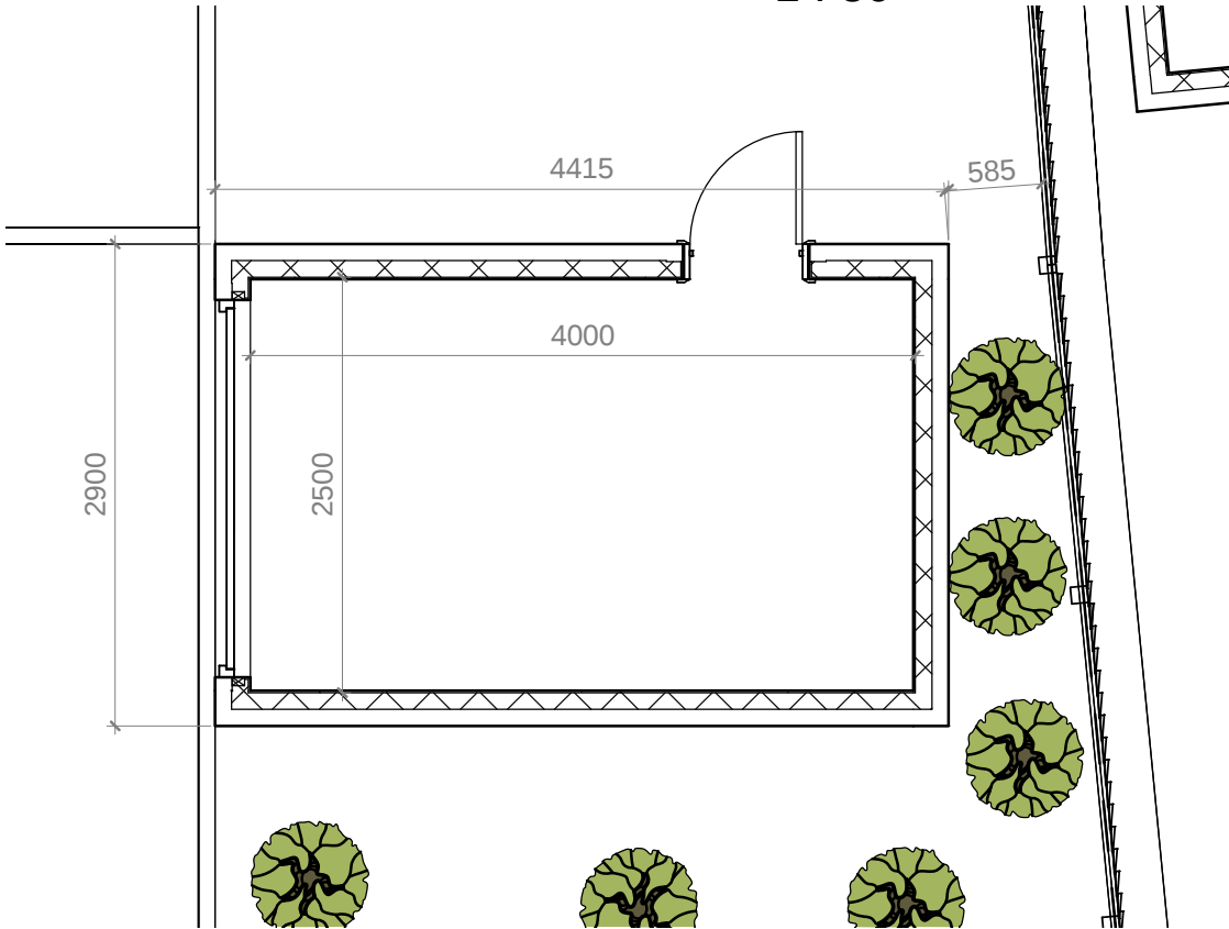
proposed plan view 1 : 50
