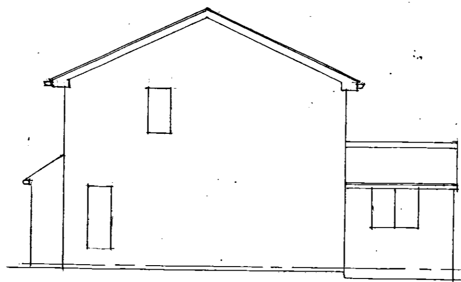
EXIST. WEST ELEVATION (SIDE)
