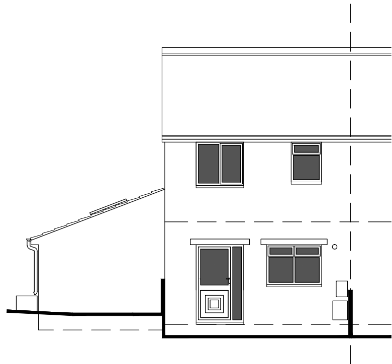
ELEVATION FACING NORTH-WEST
