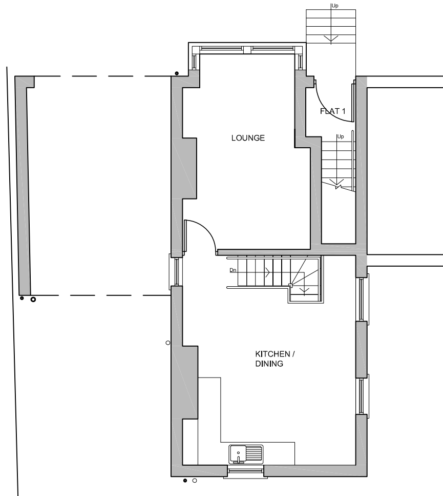
UPPER GROUND FLOOR PLAN
