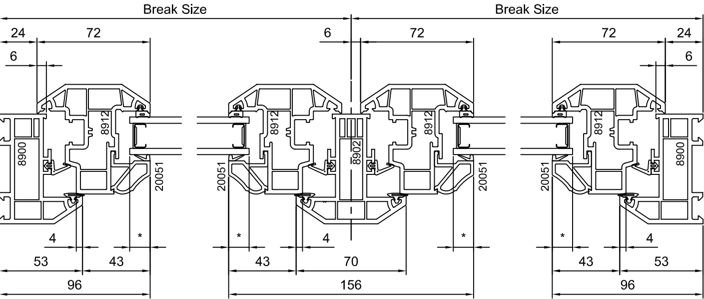
Section C-C
