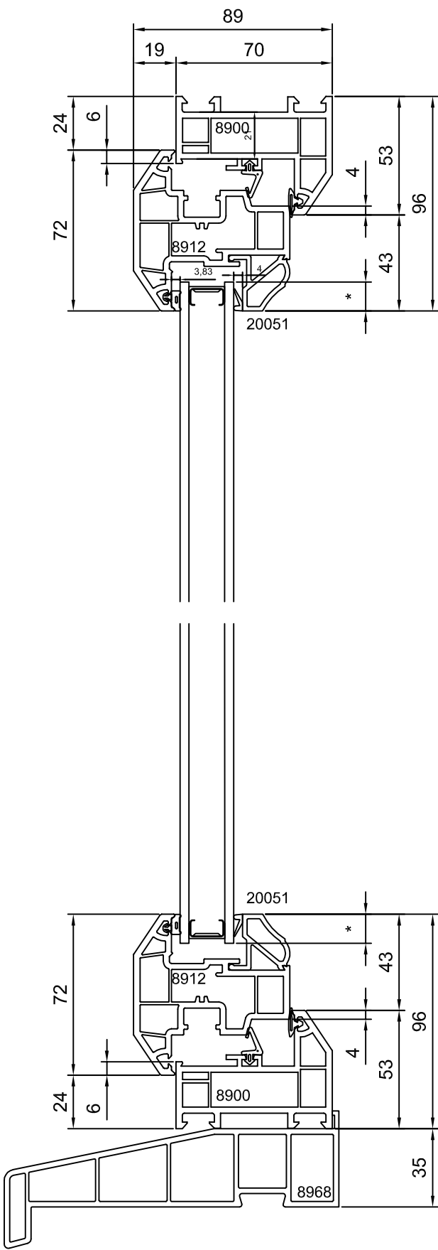
Section B-B
