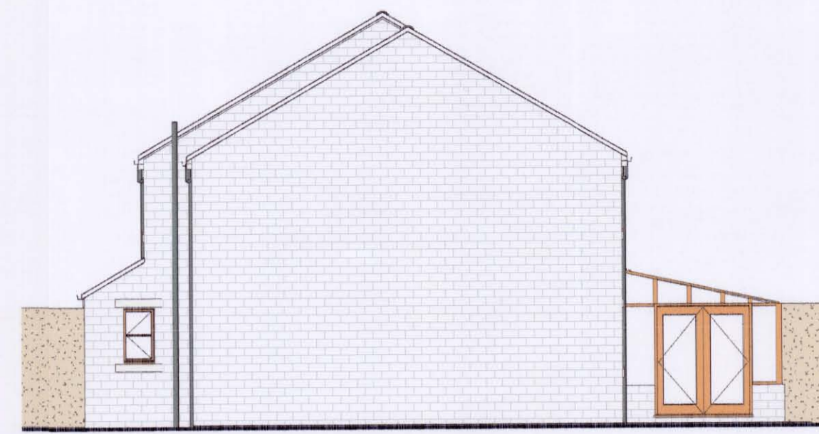
Proposed Side Elevation N 1:100
