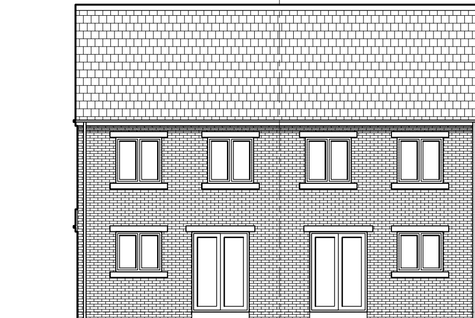
Rear Elevation
