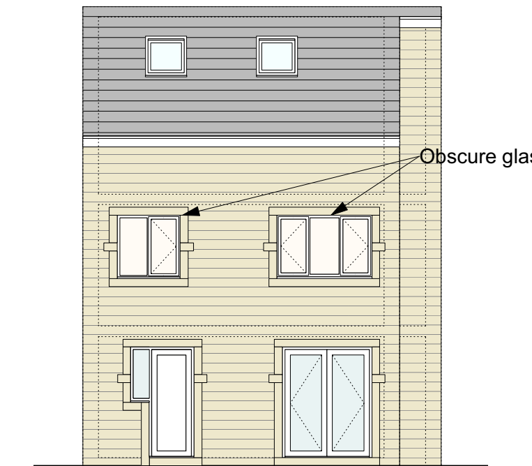
Rear Elevation As Proposed Scale 1:100 0m 1m 2m 3m 4m 5m
