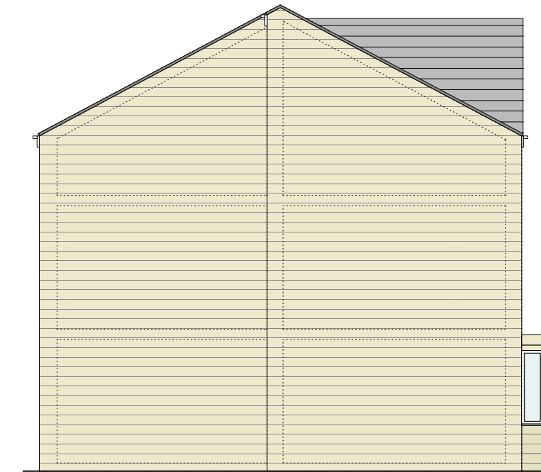
Side Elevation As Proposed Scale 1:100 0m 1m 2m 3m 4m 5m
