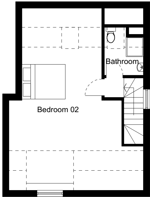
Second Floor Plan As Proposed Scale 1:100 0m 1m 2m 3m 4m 5m
