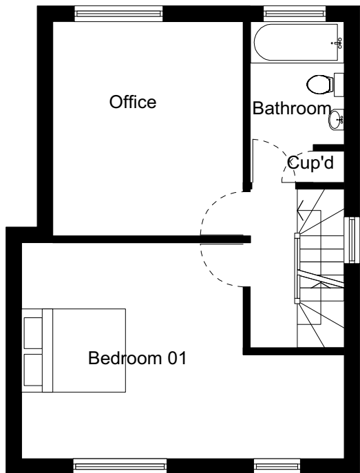
First Floor Plan As Proposed Scale 1:100 0m 1m 2m 3m 4m 5m
