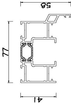
108.0933 Outer Frame Head and Jamb
