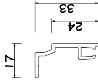
108.0990 Supporting profile Brush
