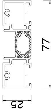
108.0934 Outer Flush Bottom
