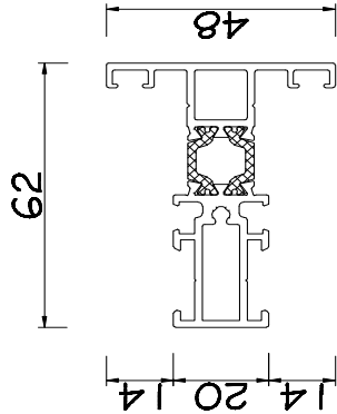
002.1753 Transom / Closer
