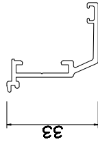
108.0992 Butt Strip Profile
