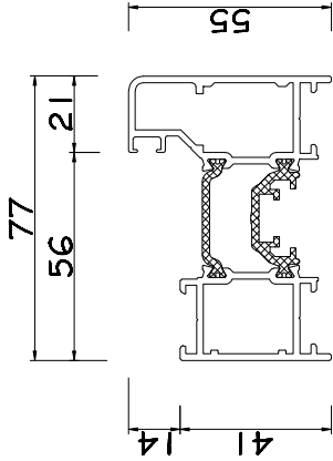
005.6327 Slim Sash
