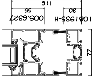
Alternative Bottom frame detail - Open Out
