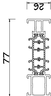
108.0896 26mm Add on
