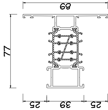
108.0120 Transom
