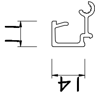
002.0677 36mm Bead
