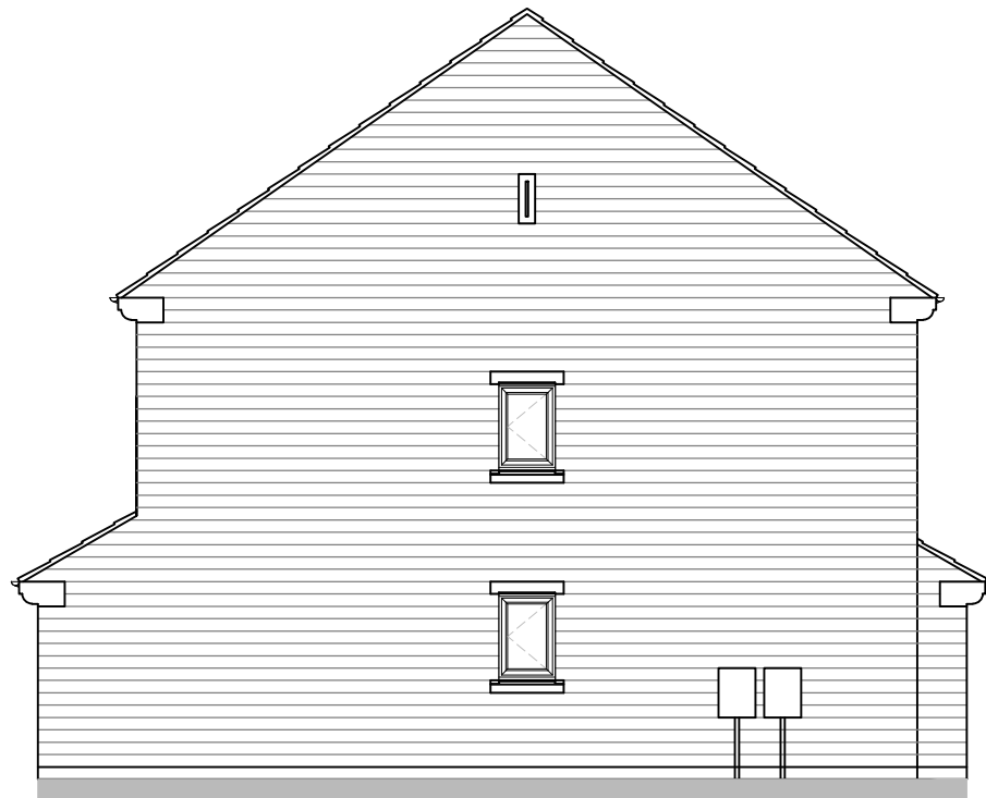
SIDE ELEVATION PLOT 9
