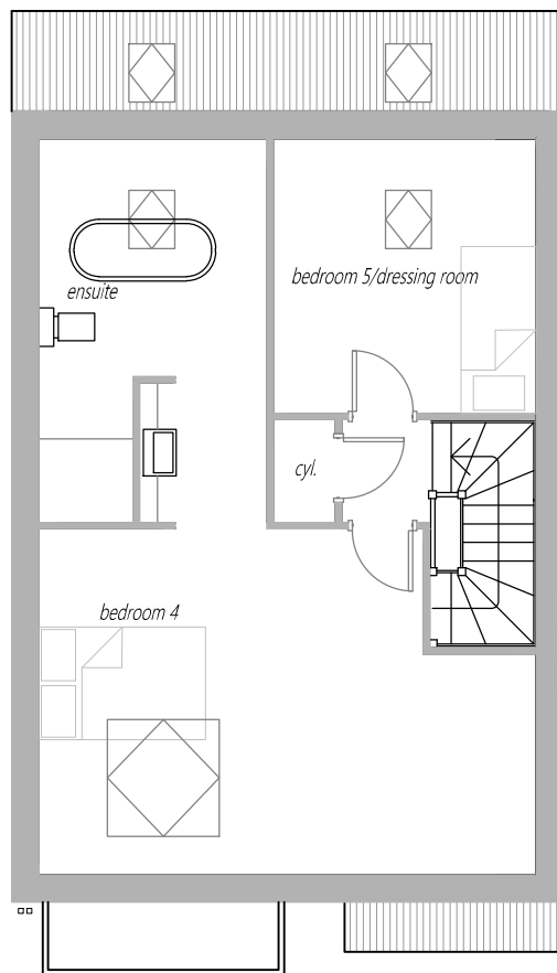
SECOND FLOOR
