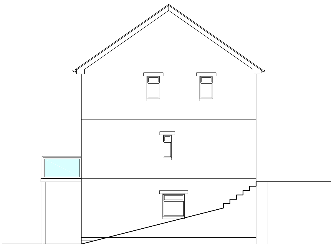
NORTH ELEVATION
