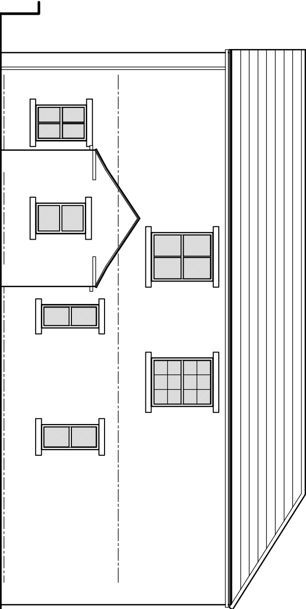
REAR ELEVATION - EXISTING 1:100
