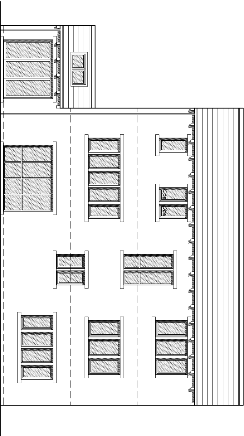
Rear Elevation
