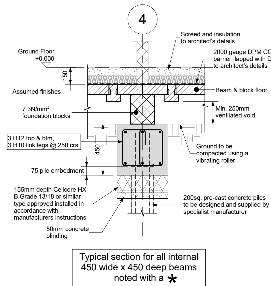
C Typical Section 1 : 20
