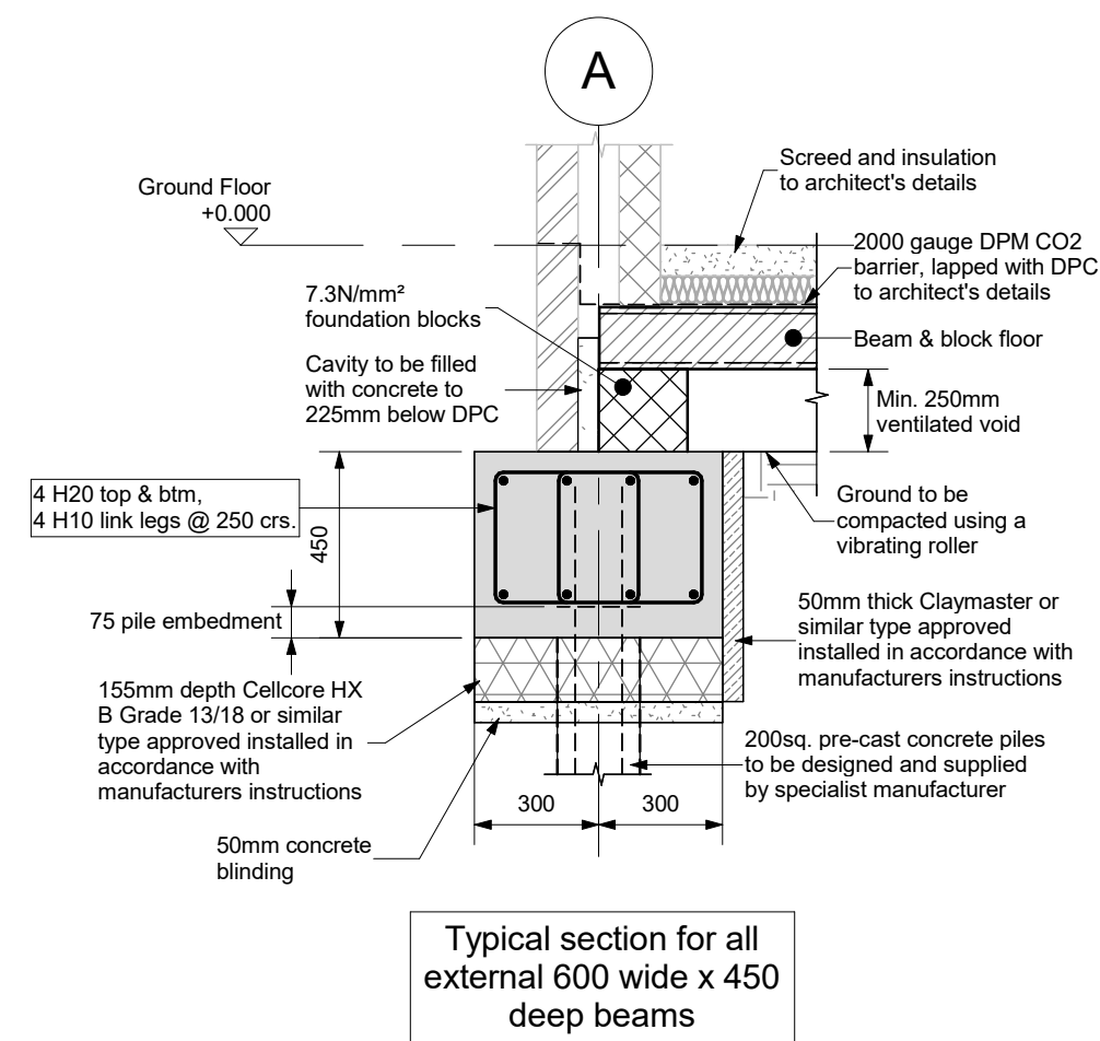
A Typical Section 1 : 20
