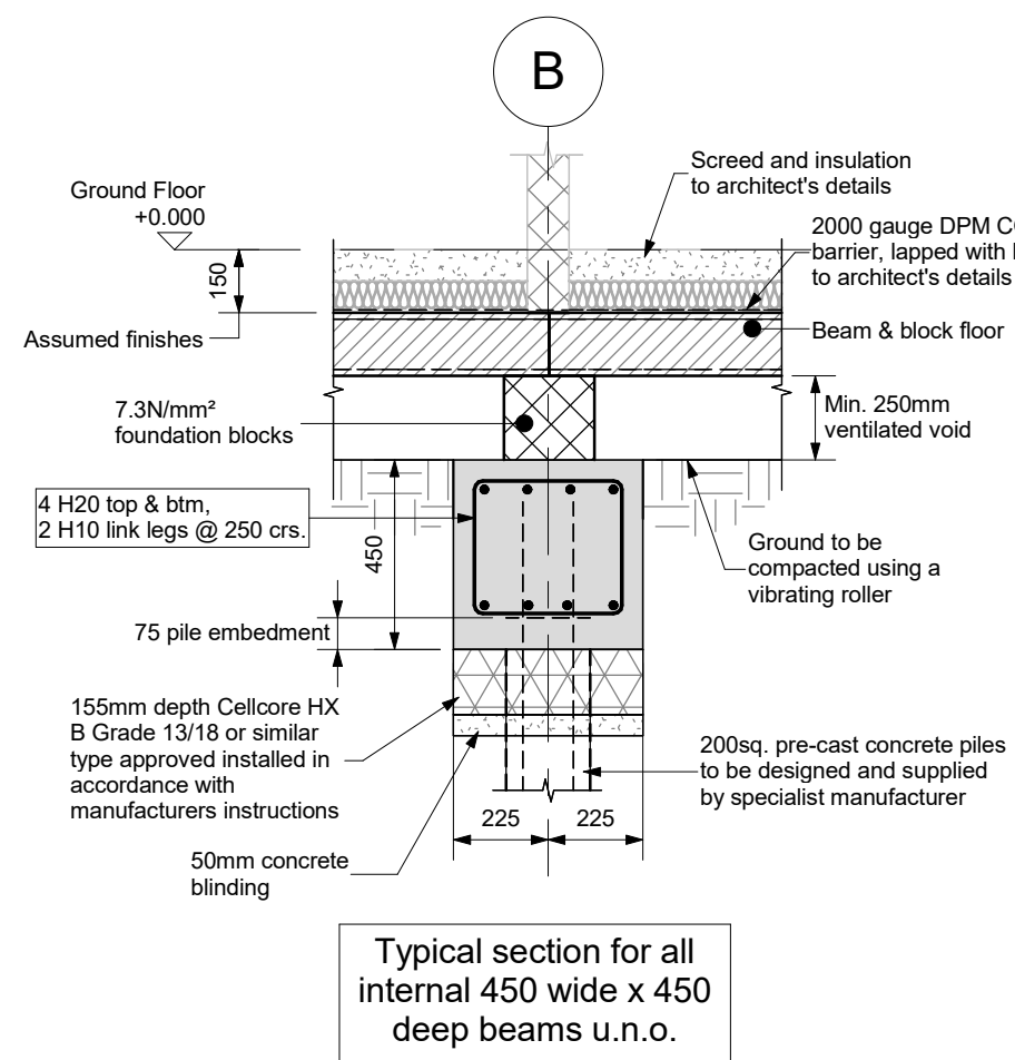
B Typical Section 1 : 20
