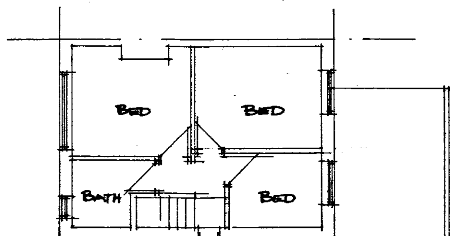
FIRST 1:100
