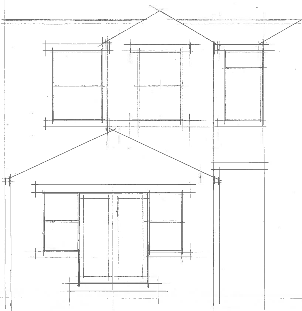
REAR ELEVATION
