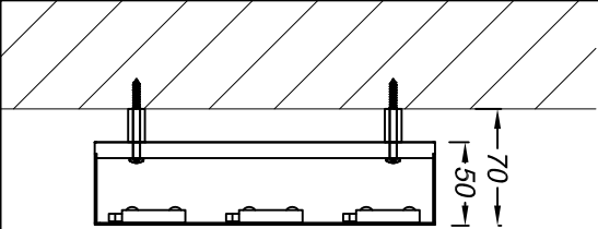
Section C-C through the text Scale 1:5
