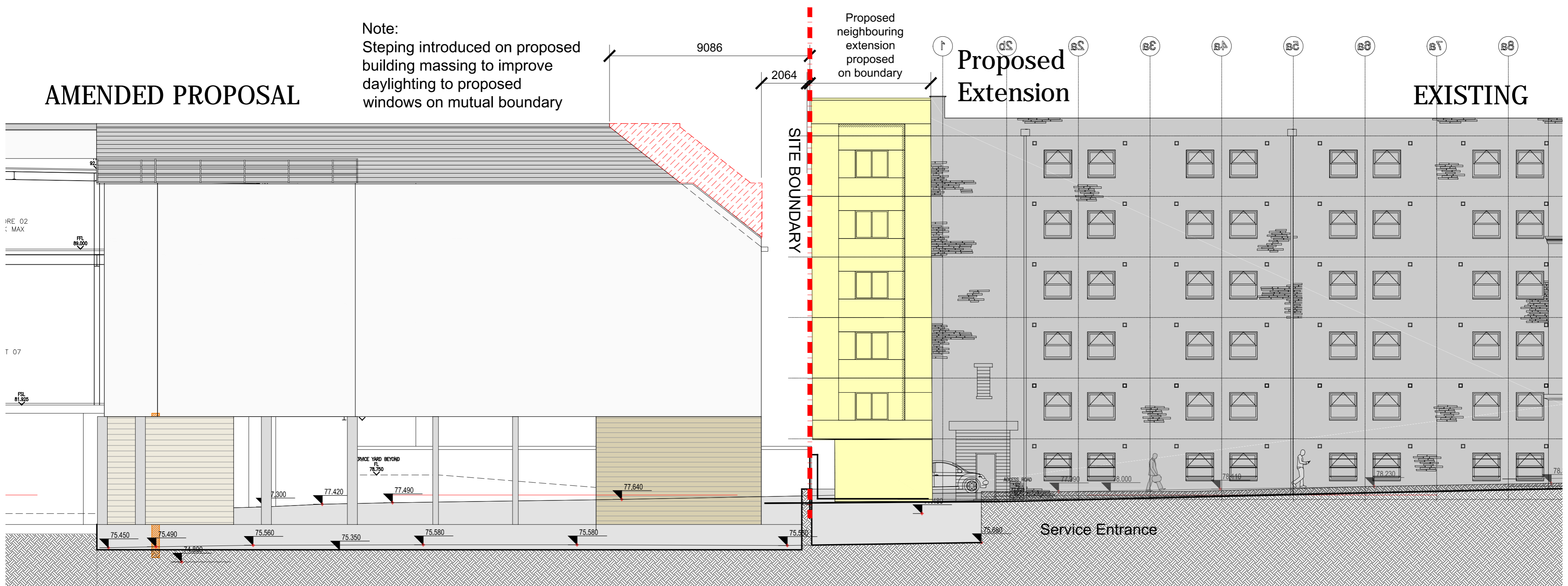
STAGE 3 - Amended Proposed Elevation, showing amended roof and gable profile to neighbouring (unbuilt) Planning Consent
