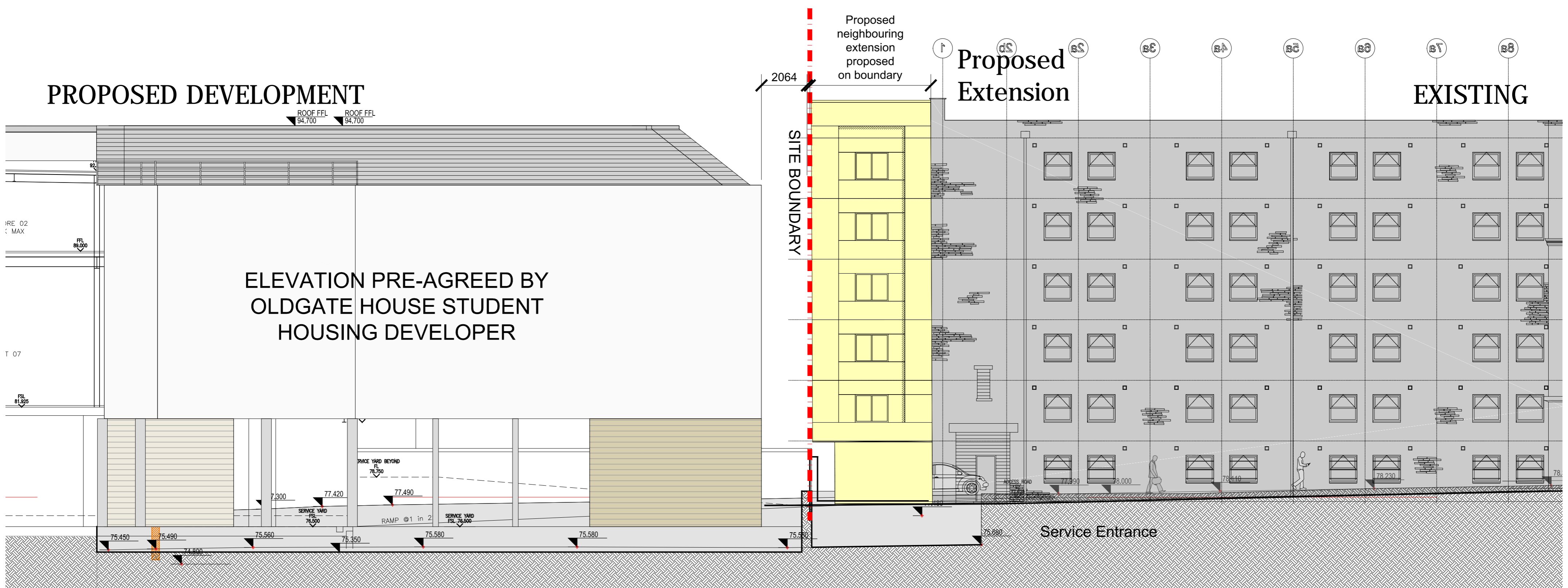
STAGE 2 - Original Proposed Elevation, showing neighbouring (unbuilt) Planning Consent
