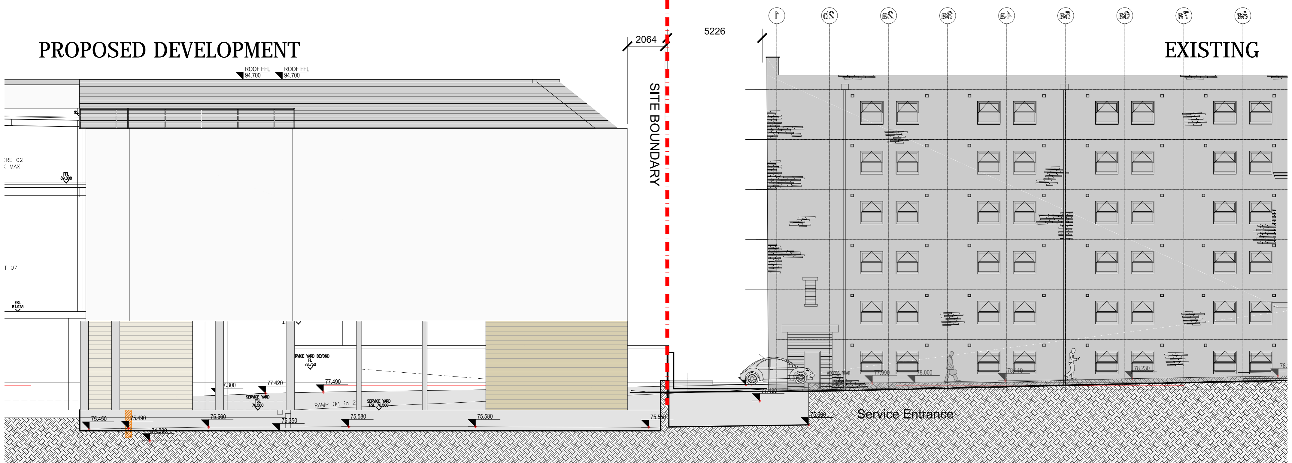
STAGE 1 - Original Proposed Elevation
