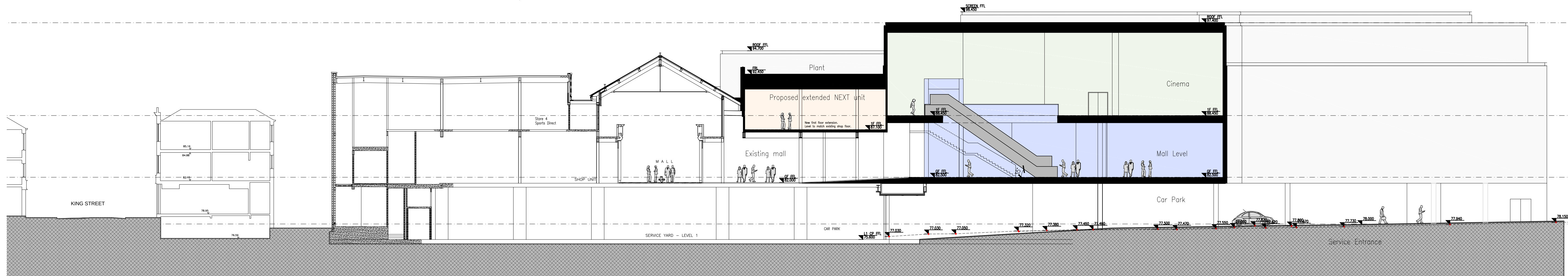
PROPOSED SECTION B-B, THRU NEW RETAIL EXTENSION & CINEMA
