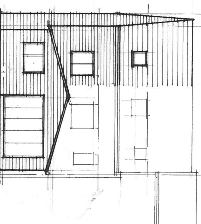
REAR 1:100
