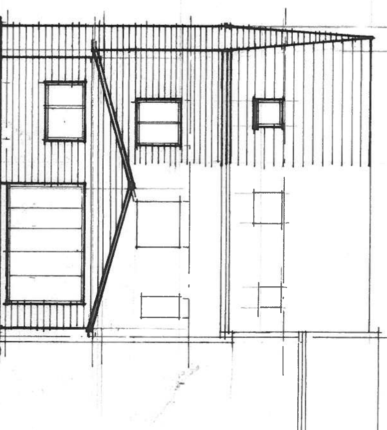
REAR 1:100
