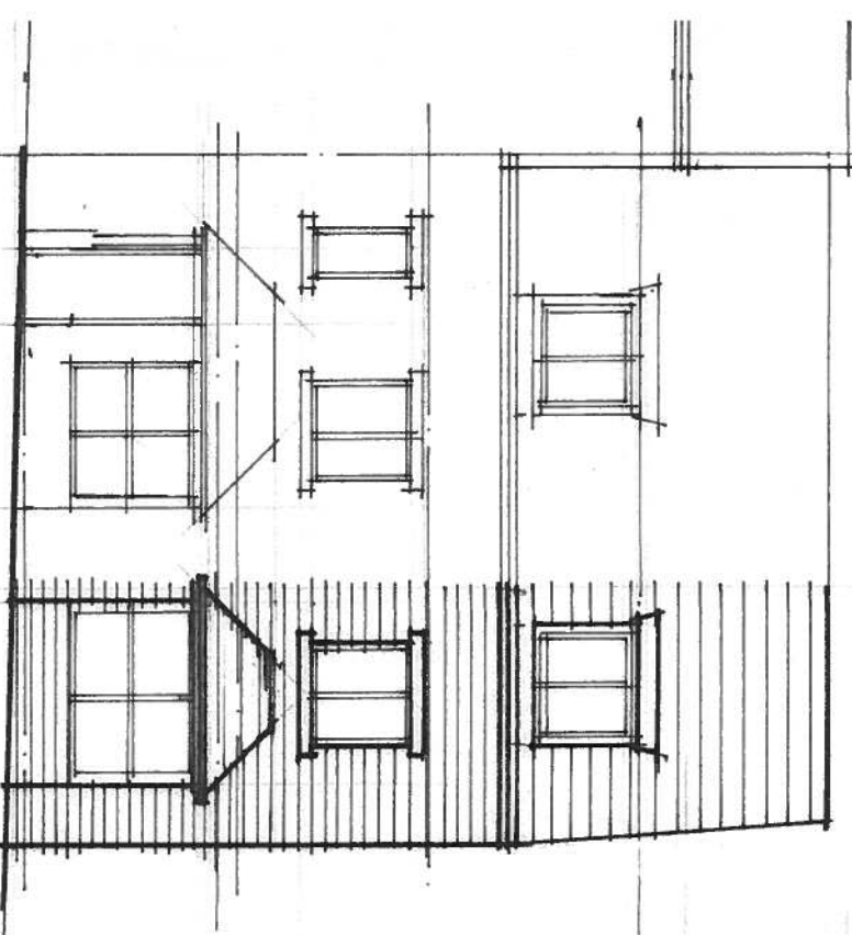
FRONT 1:100
