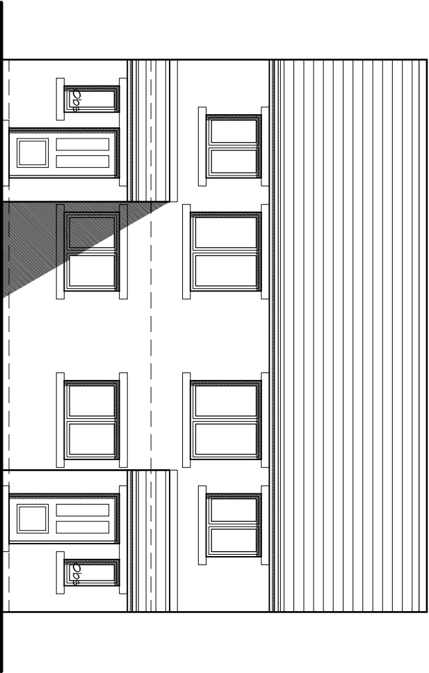
Front Elevation
