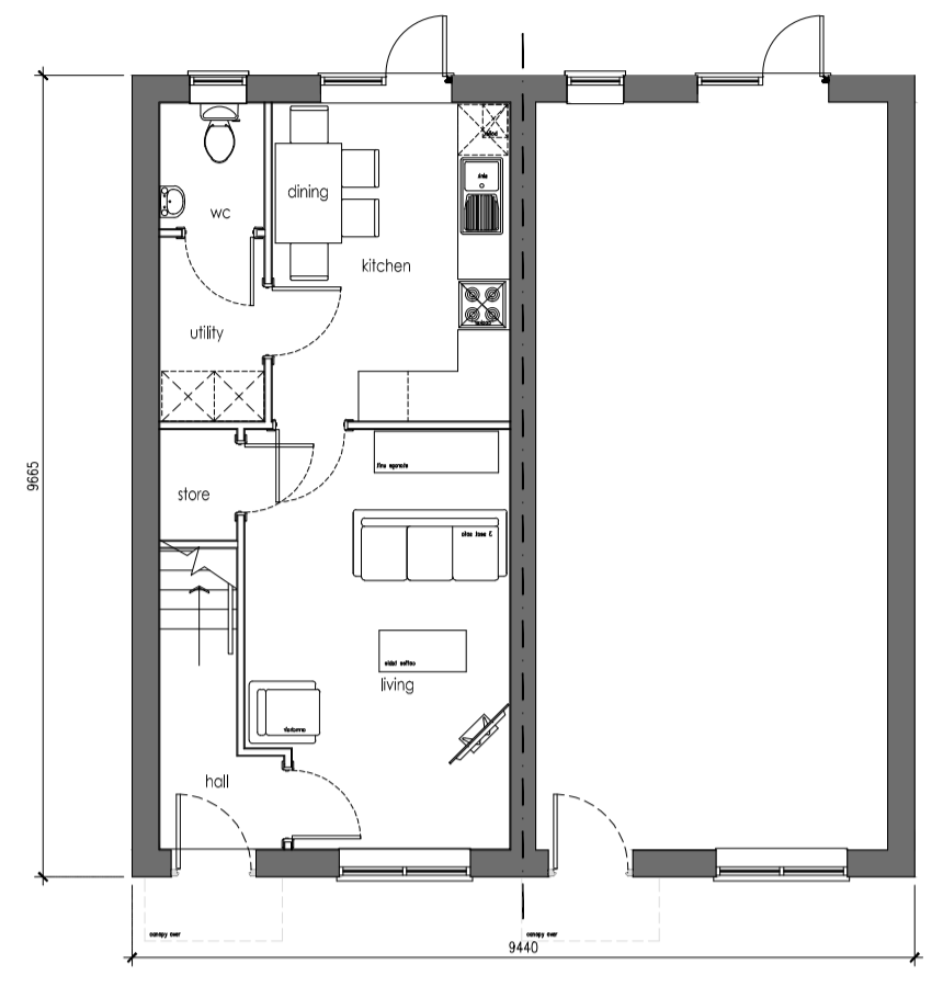
Ground floor plan GIA = 38 sqm
