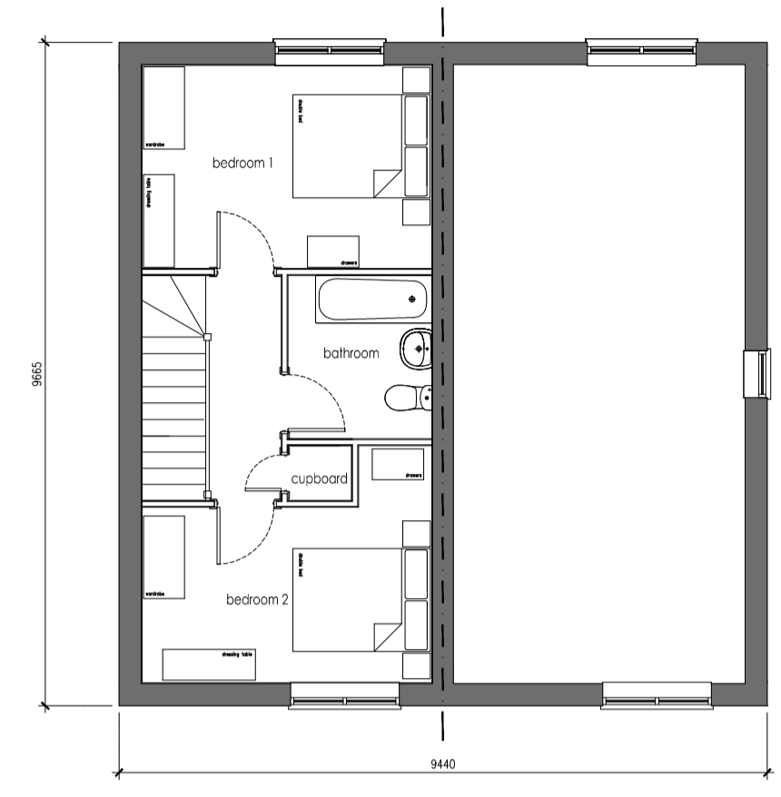
First floor plan GIA = 38 sqm
