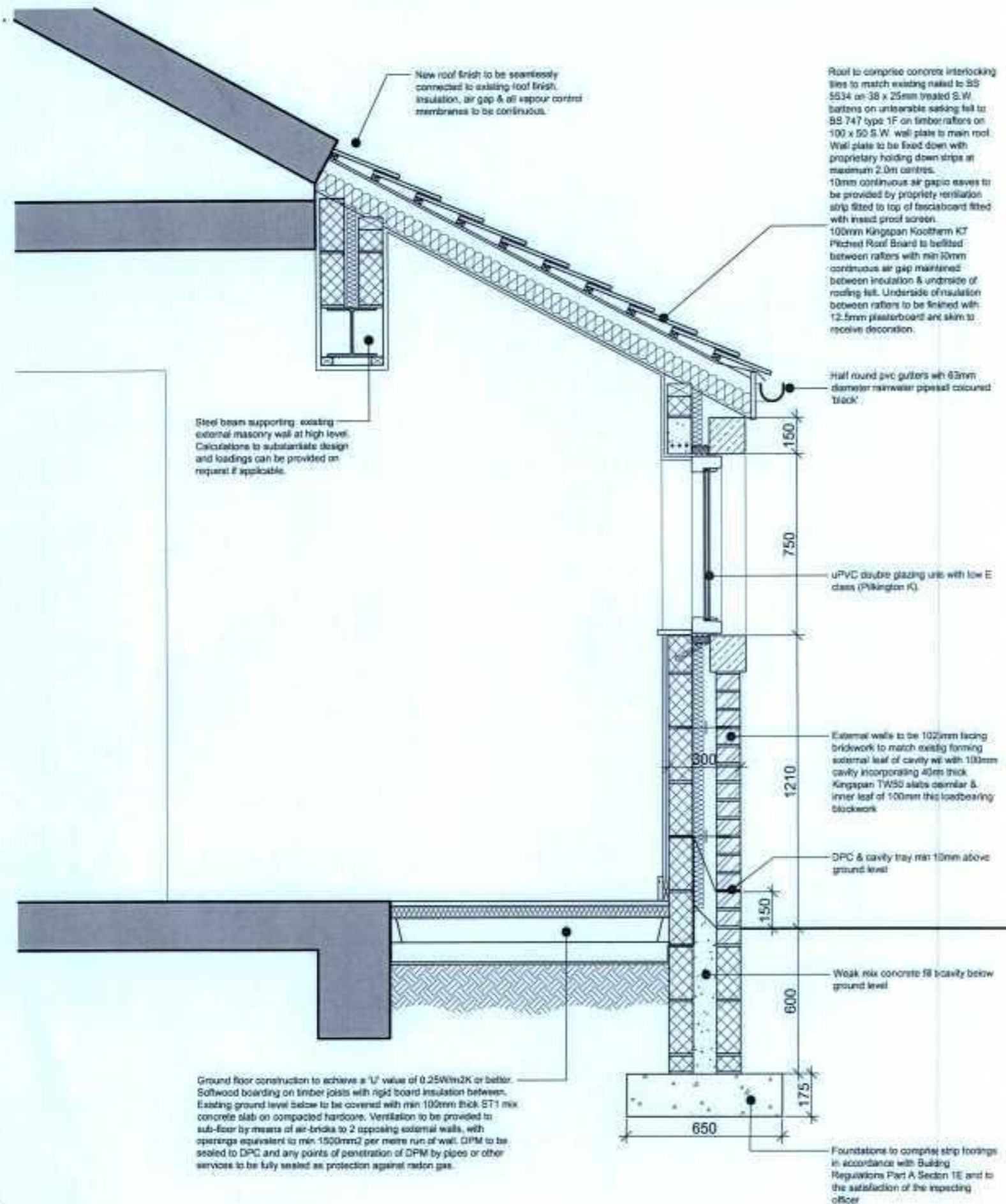
DETAILED SECTION SCALE 1:20
