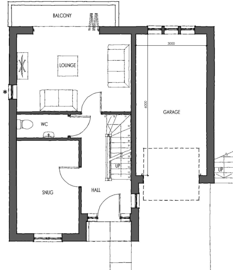
UPPER GROUND FLOOR PLAN * LOUNGE SIDE WINDOW TO PLOT 12 ONLY
