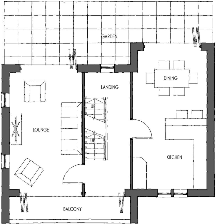
UPPER GROUND FLOOR PLAN
