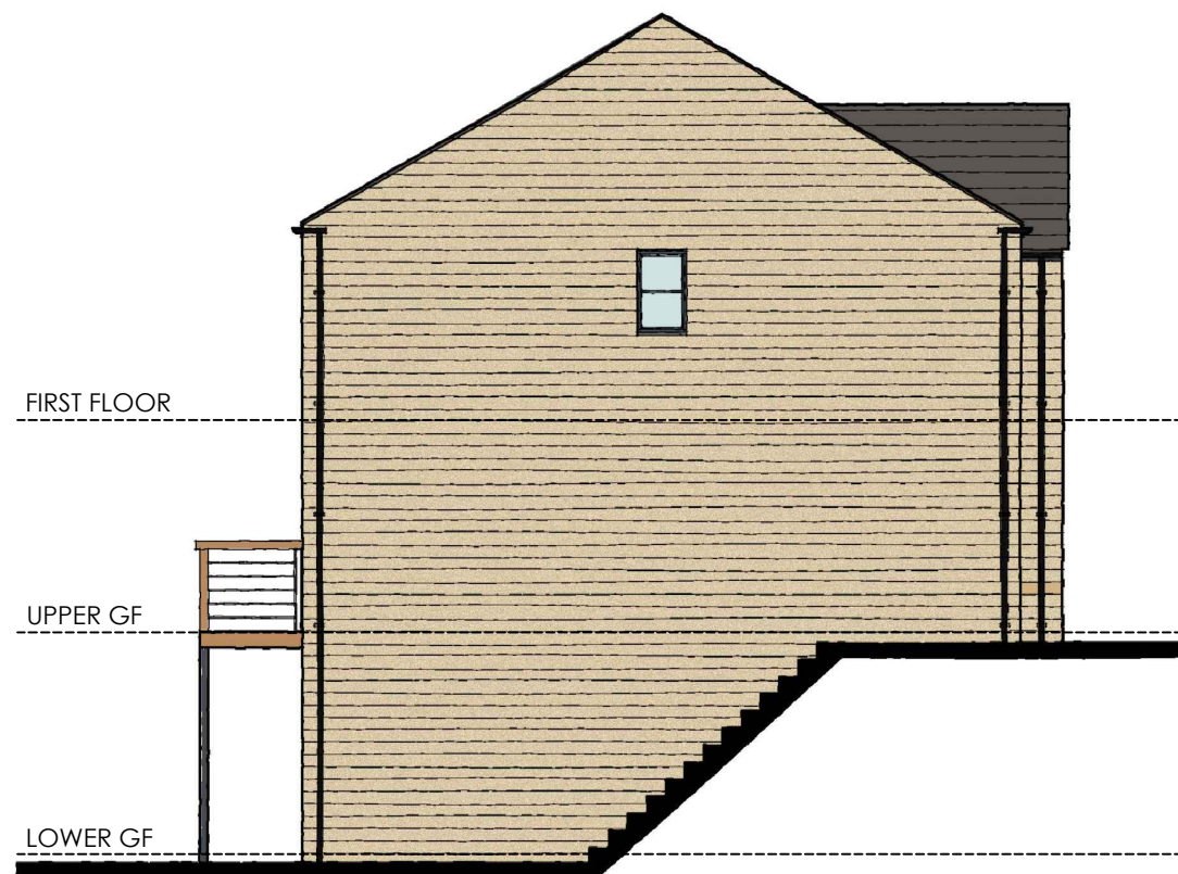
PLOT 1 SIDE ELEVATION
