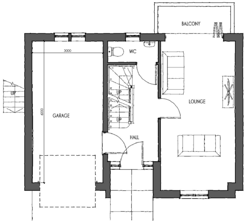
UPPER GROUND FLOOR PLAN
