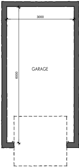
FLOOR PLAN
