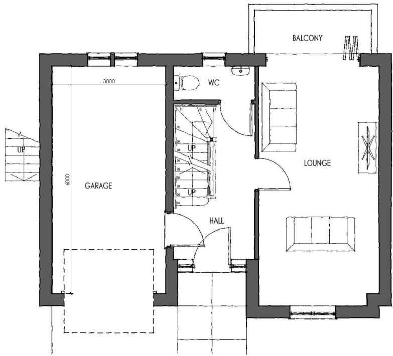
UPPER GROUND FLOOR PLAN
