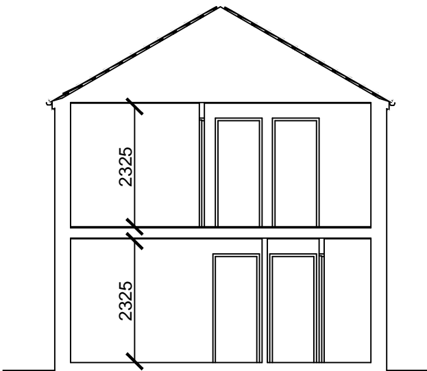
TYPICAL SECTION
